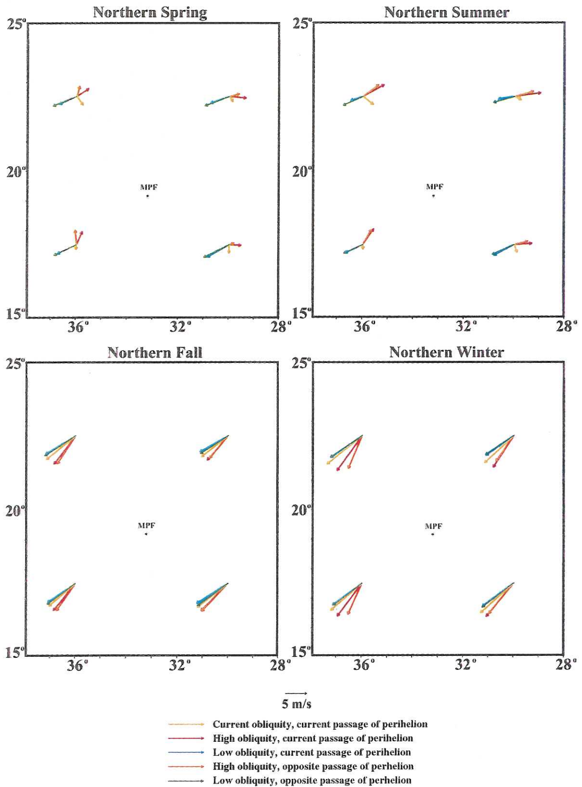
Plate 2. Winds at the Mars Pathfinder landing site for differing obliquity and perihelion states. Note how the strongest surface winds always come from the northeast in the northern fall and winter regardless of astronomical oscillations.
