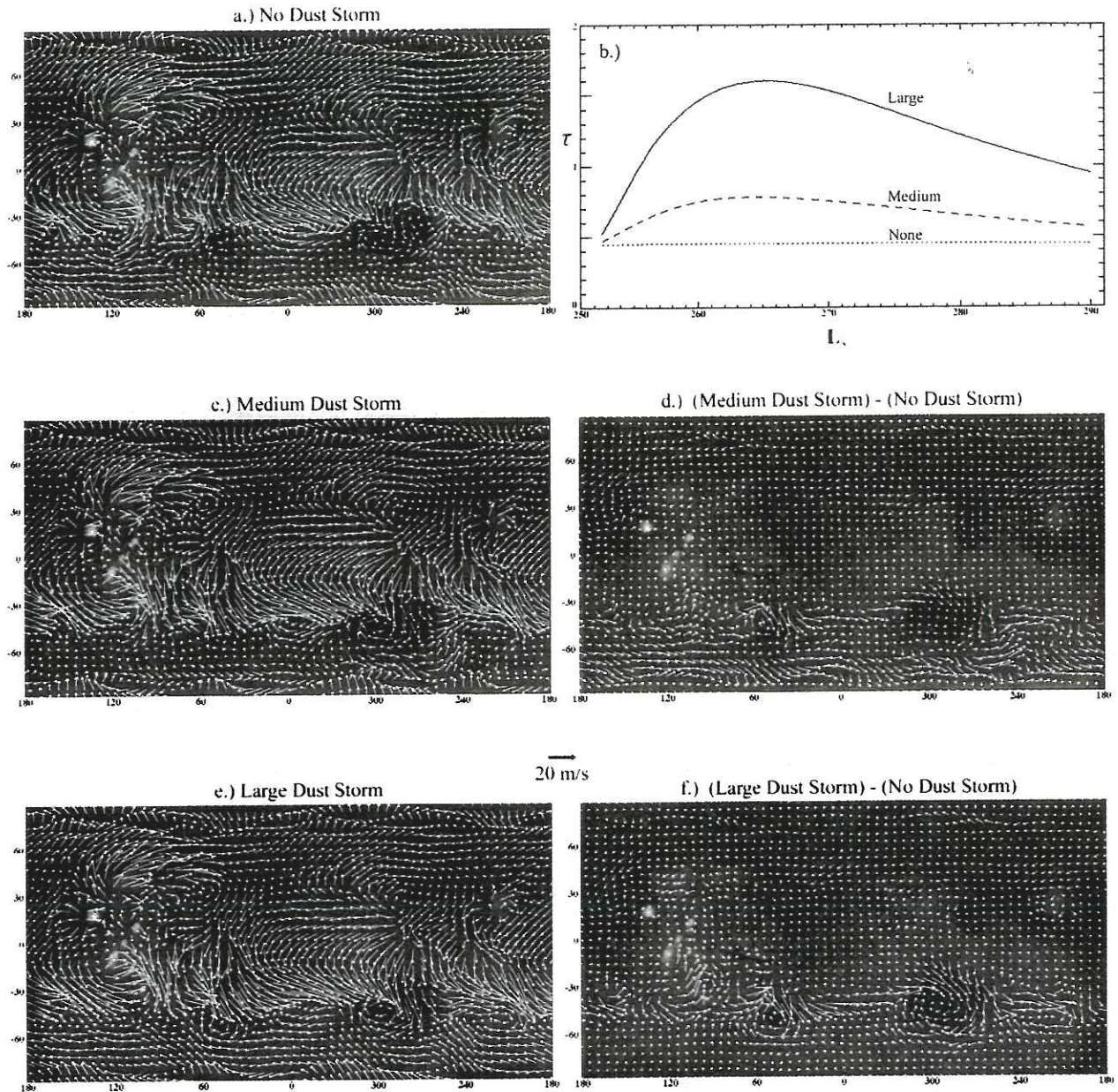
Figure 2. (a) Global surface winds averaged from L_s = 251^\circ to L_s = 291^\circ in a year with no dust storm. (b) Average global dust optical depth as a function of time for the three storm cases shown in this figure. (c) Global surface winds over the same time period in a year with moderate dust lifting between 20^\circ\text{S} and 40^\circ\text{S} (maximum dust opacity \approx 1.6 ). (d) Changes in wind strength and direction of the moderate storm case relative to the non-dusty case. (e) Global surface winds over the same time period in a year with strong dust lifting between 20^\circ\text{S} and 40^\circ\text{S} (maximum dust opacity \approx 5 ). (f) Changes in wind strength and direction of the strong storm case relative to the non-dusty case.
