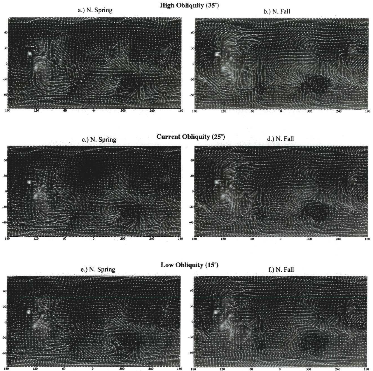
Figure 5. Global surface winds at high obliquity ( 35^\circ ) averaged over (a) northern spring and (b) northern fall. Global surface winds at the current obliquity ( 25^\circ ) averaged over (c) northern spring and (d) northern fall. Global surface winds at low obliquity ( 15^\circ ) averaged over (e) northern spring and (f) northern fall.
