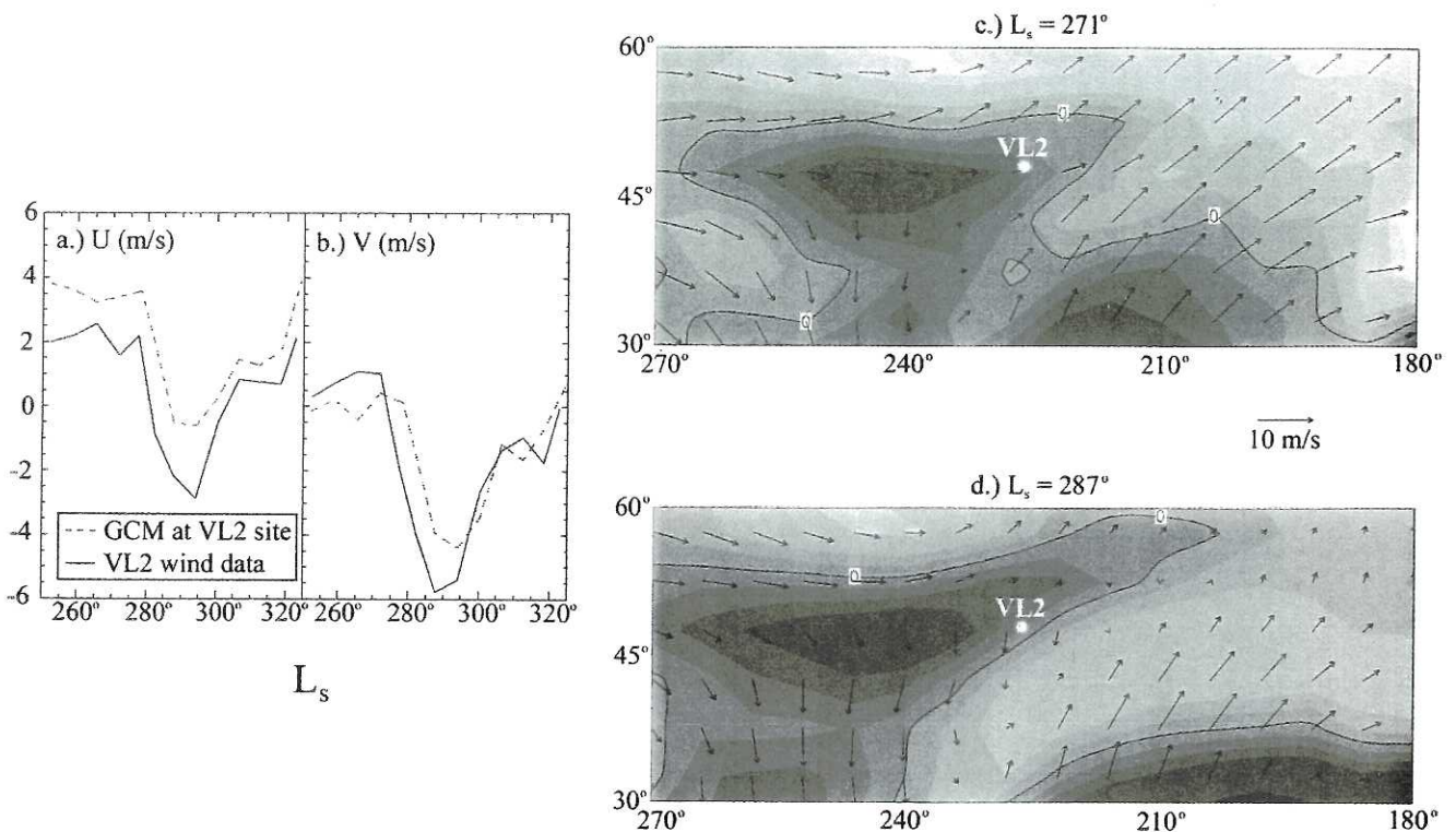
Figure 3. A comparison of (a) zonal (westerly) and (b) meridional (southerly) winds measured by Viking Lander 2 and predicted by the general circulation model (GCM) over the lander site. Wind speed, direction, and divergence are shown (c) before the 1977b dust storm at L_s = 271^\circ and (d) during the dust storm at L_s = 287^\circ . Convergence (upwelling) is shown as light shades; divergence (downwelling) is shown as darker shades. The line labeled 0 delineates the change from convergence to divergence.
