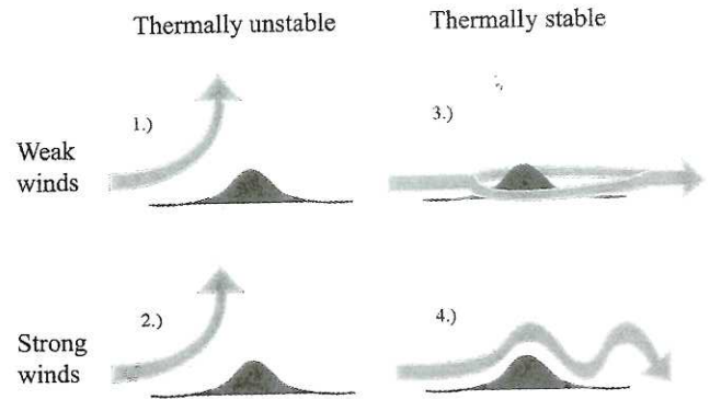
Figure 4. The four possible situations produced by horizontal flow over an obstacle.
