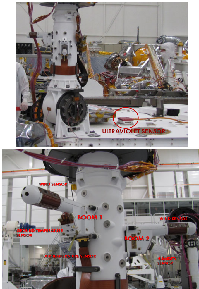
Fig. 4 Images taken during the REMS integration show the position of the REMS sensors. Top image shows the location of Booms 1 and 2 and UVS. Bottom image is a close-up of both booms. (Credit: NASA/JPL)
