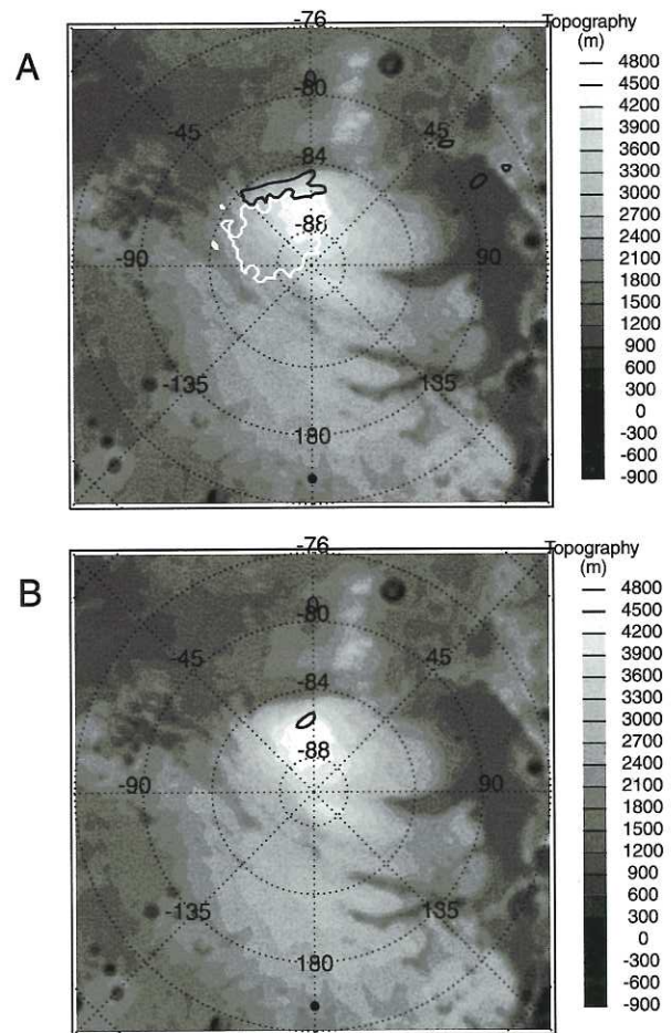
Figure 8. Wind stresses in the south polar region at L_s = 310^\circ . Topography is shown by the gray shading in the background. The extent of the seasonal cap is shown by the white line. Surface wind stress is contoured by the thick black lines in intervals of 0.032 Pa. The small black circle is the longitude of local noon, in this case, 180^\circ\text{E} . (a) "Base" simulation. (b) Simulation where the thermal effects of the residual cap (i.e., \text{CO}_2 ice, thermal inertia, and albedo signature) have been removed.
