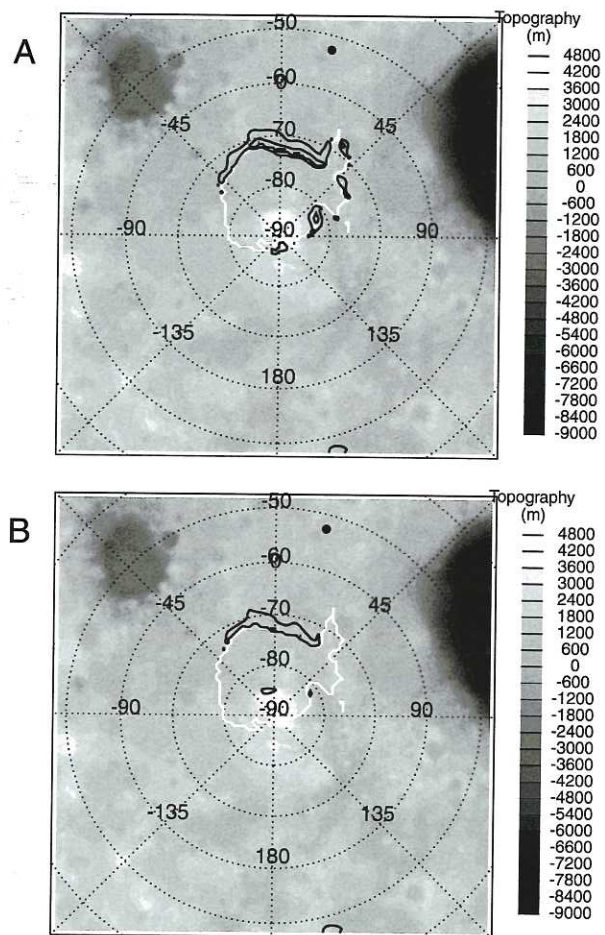
Figure 6. Wind stresses in the south polar region at L_s = 255^\circ . Topography is shown by the gray shading in the background. The extent of the seasonal cap is shown by the white line. Surface wind stress is contoured by the thick black lines in intervals of 0.032 Pa. The small black circle is the longitude of local noon, in this case, 15^\circ\text{E} . (a) “Base” simulation. (b) Simulation where the surface covering of \text{CO}_2 ice has been removed.
